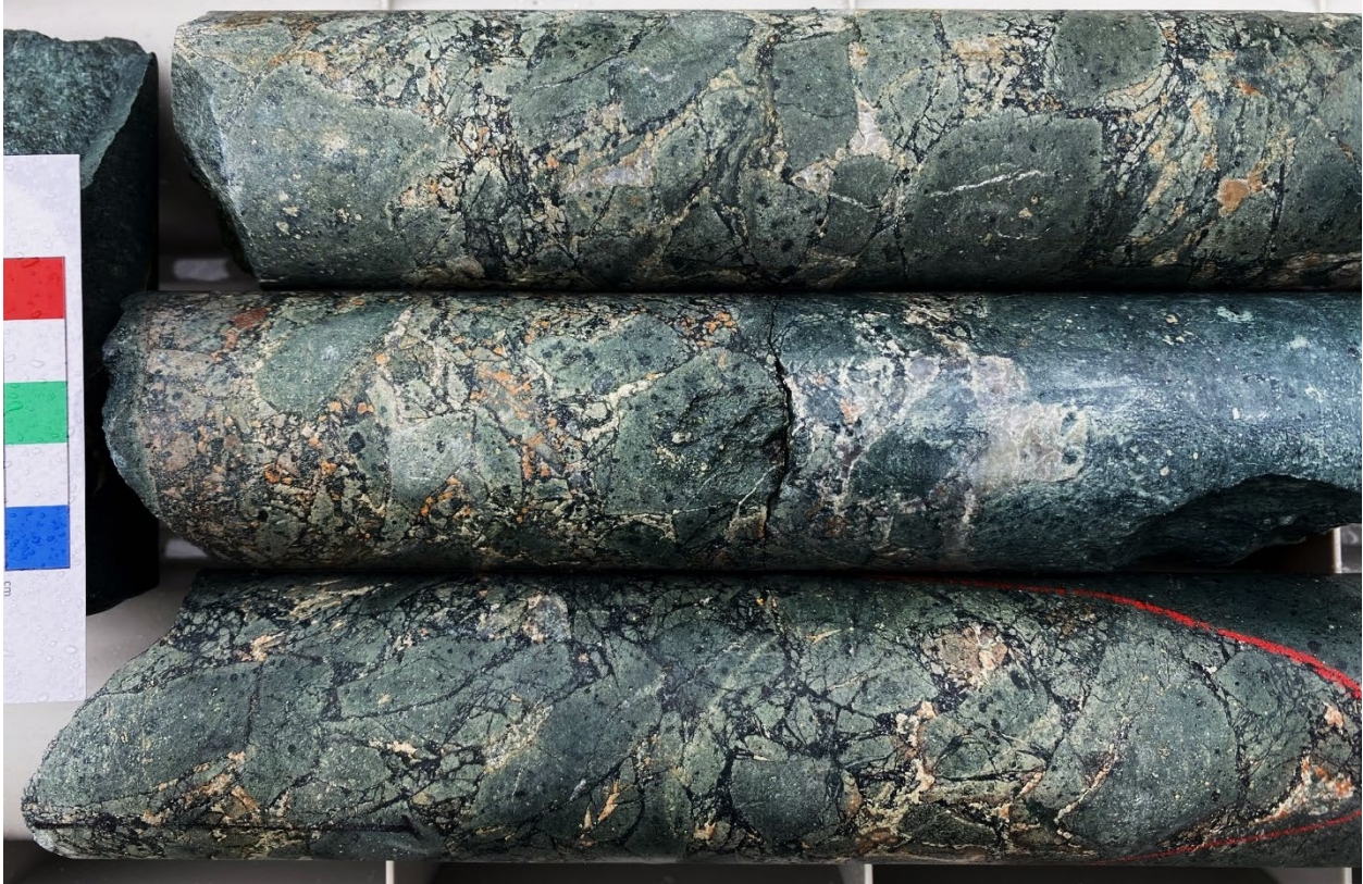
Photo 3. Nine Mile drill hole MYLDH001 183.5, 186.2 and 188.4 meters. Quartz-carbonate-chlorite cemented hydrothermal breccia. Breccias such as these are definitive indicators of hydrothermal fluid flow zones and are considered encouraging signs from a first-pass drill program.
